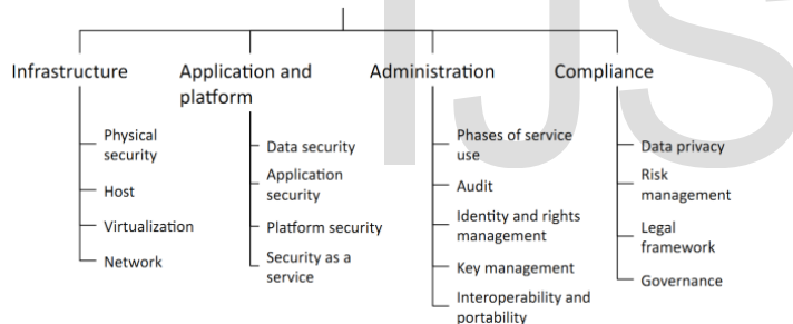
Fig. 3.1: Taxonomy of security aspects within cloud computing systems [8]
